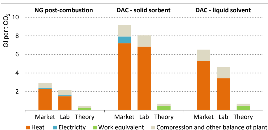
Figure 4.10 ► Best-in-class energy consumption for CCUS technologies by context
