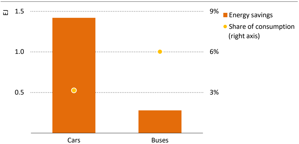
Figure 3.15 ▶ Energy savings in passenger vehicles in the Widespread Adoption Case, 2035
